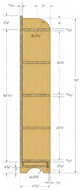
SIDE SECTION
